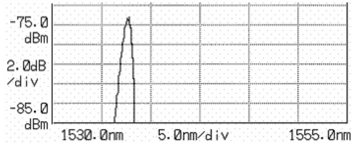
Fig. 12. 1532 nm stack with internal grating stabilization, output spectrum at 175 W, showing <2 nm FWHM.
