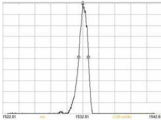
Fig. 10. 1532 nm bar with internal grating stabilization, output spectrum at 20 W, showing <math><1.6\text{ nm}</math> FWHM.
