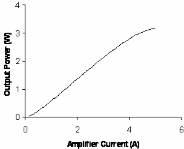
Fig. 6. Power versus current in the amplifier section for 1040 nm single frequency single mode MOPA device. Figure 7 shows the spectrum for a device at 3 Watt. The line width was measured to be < 50MHz. More than 30dB of suppression was observed. Figure 8 shows the slow axis beam quality measurement, with performance less than 1.2 times the diffraction limit.
