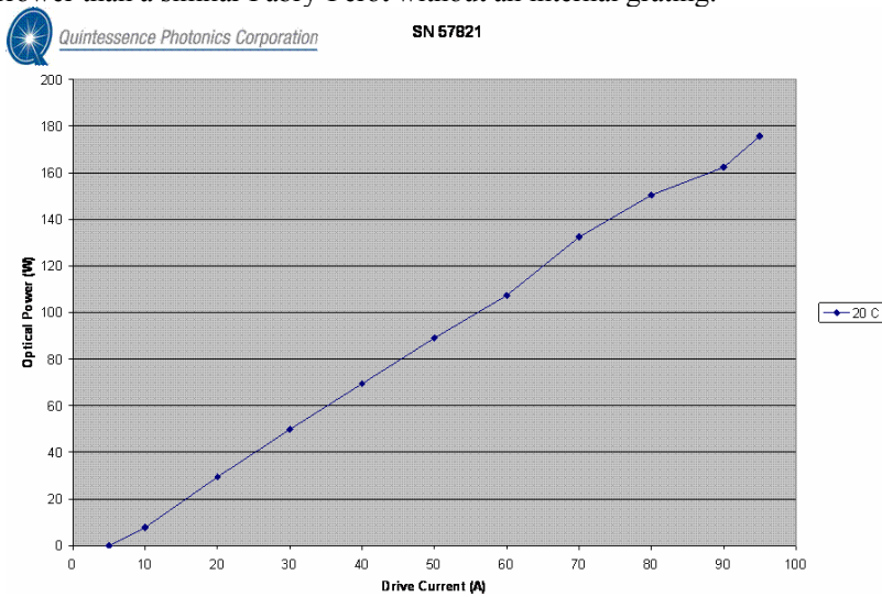
Fig. 11. 1532 nm water cooled stack with internal grating stabilization, power versus current performance
