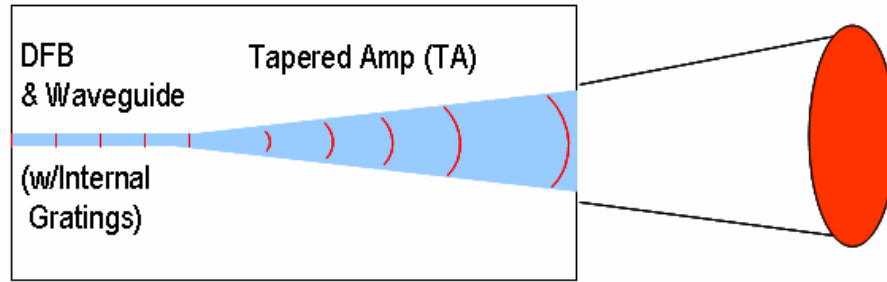
Fig. 5. Schematic of 1040 nm single frequency single mode MOPA device
