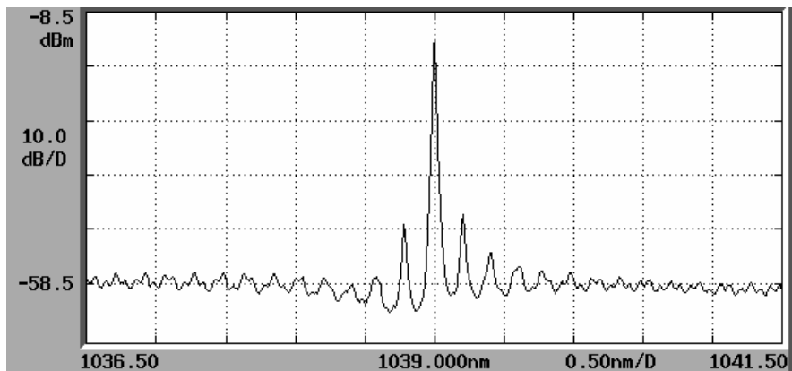
Fig. 7. Spectrum for 1040 nm single frequency single mode MOPA device.
