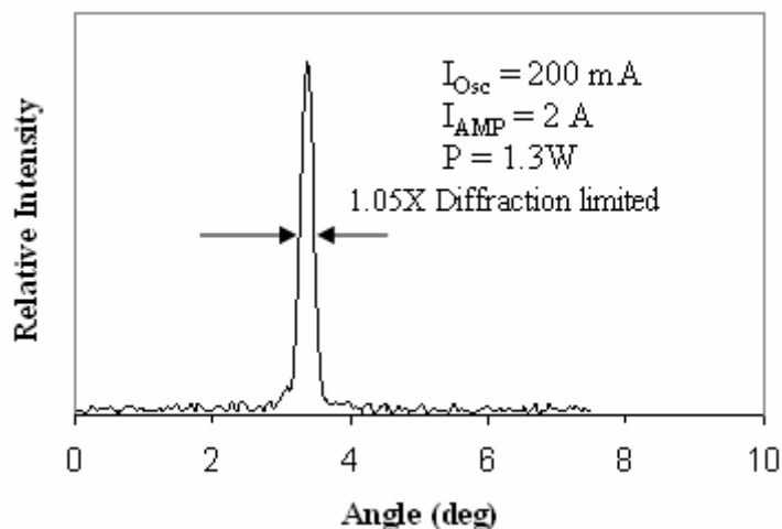
Fig. 8. Mode measurement for 1040 nm single frequency single mode MOPA device.
