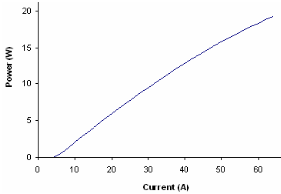
Fig. 9. 1532 nm bar with internal grating stabilization, power versus current performance
