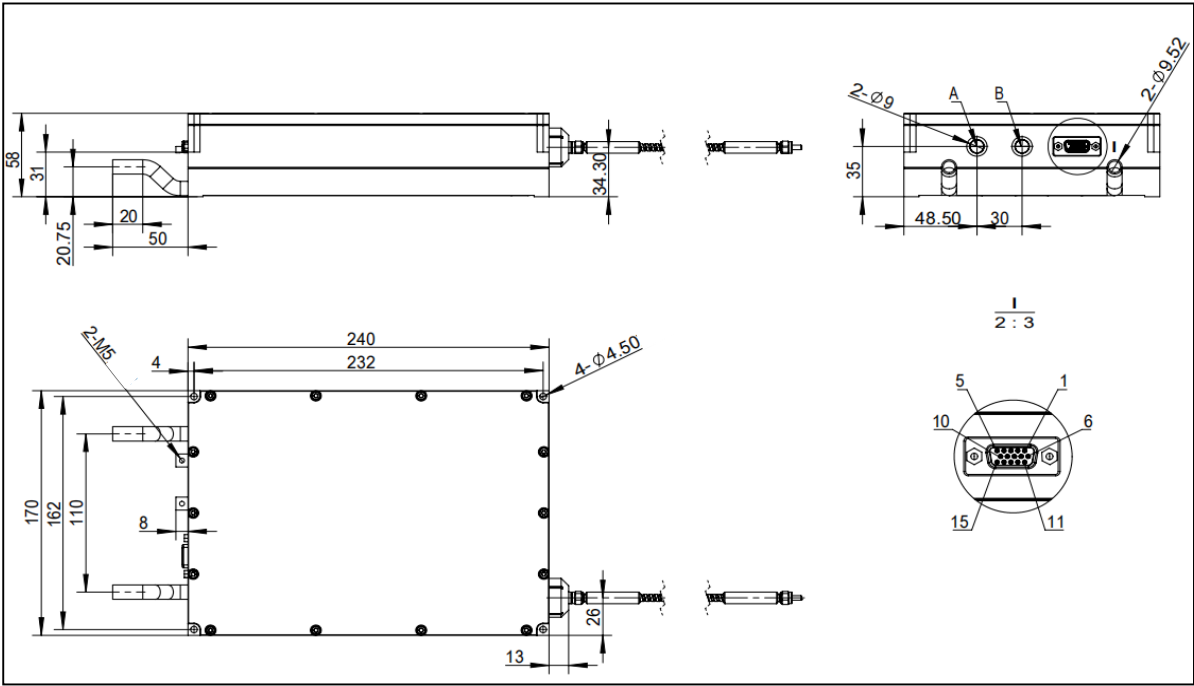
Outline Dimensions and Pin-out
