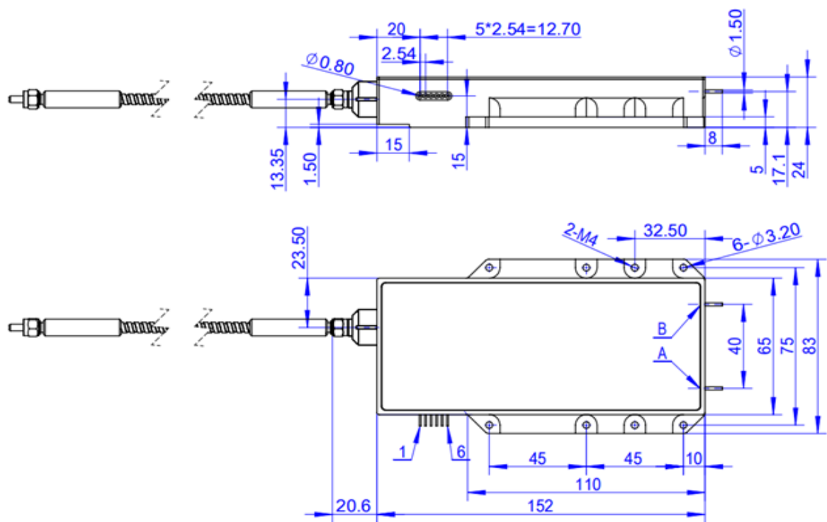
Outline Dimensions and Pin-out
